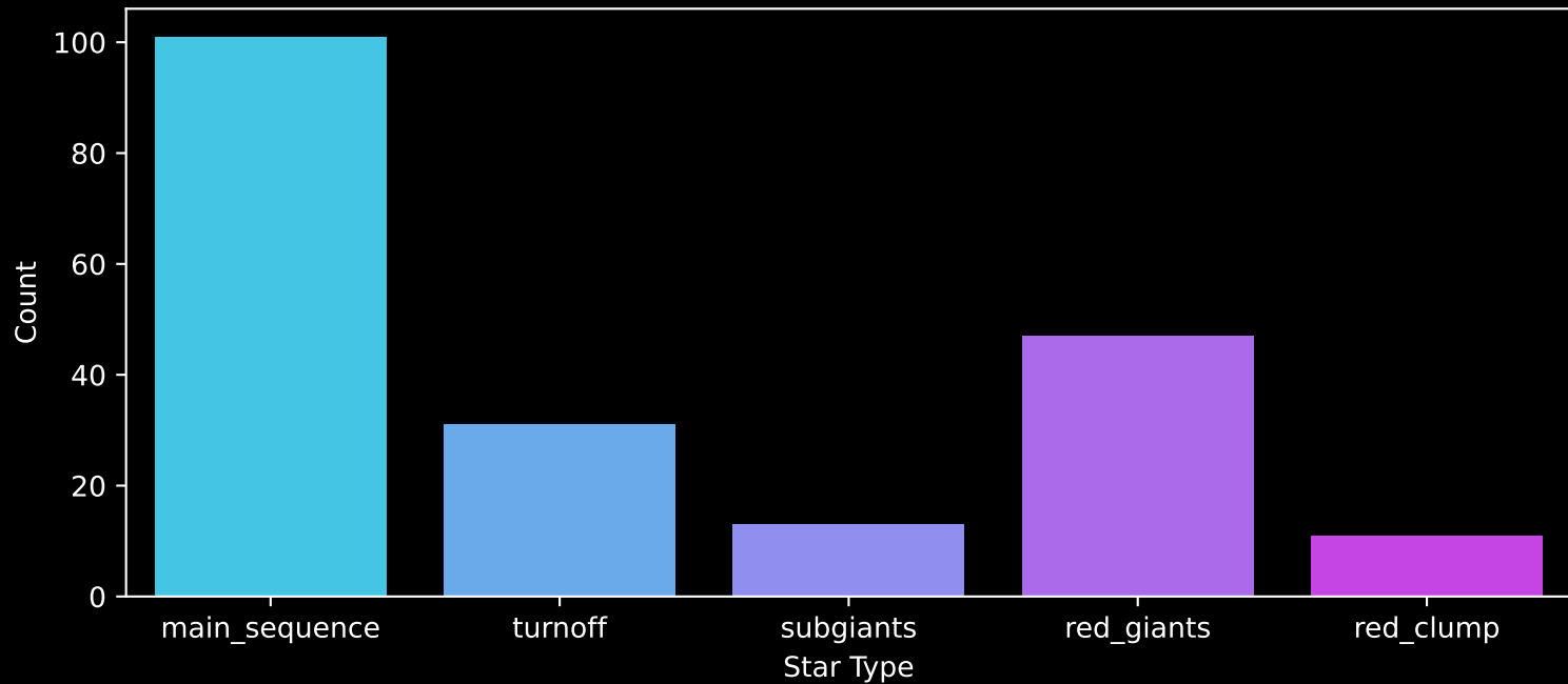
APOGEE DR17 Field: [193+34_MGA] Count plot of Star Type
