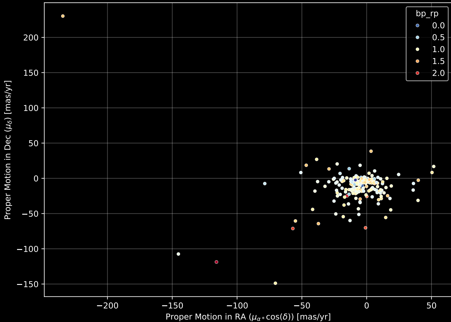
APOGEE DR17 Field: [193+34_MGA] Proper Motion Diagram (n= 203)
