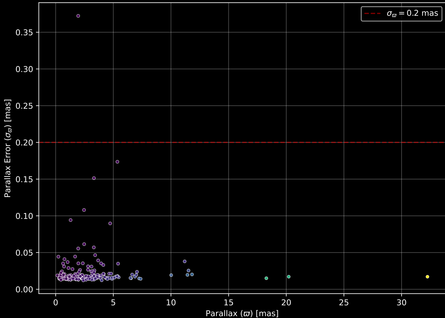
APOGEE DR17 Field: [193+34_MGA] Parallax Quality (n= 203)
