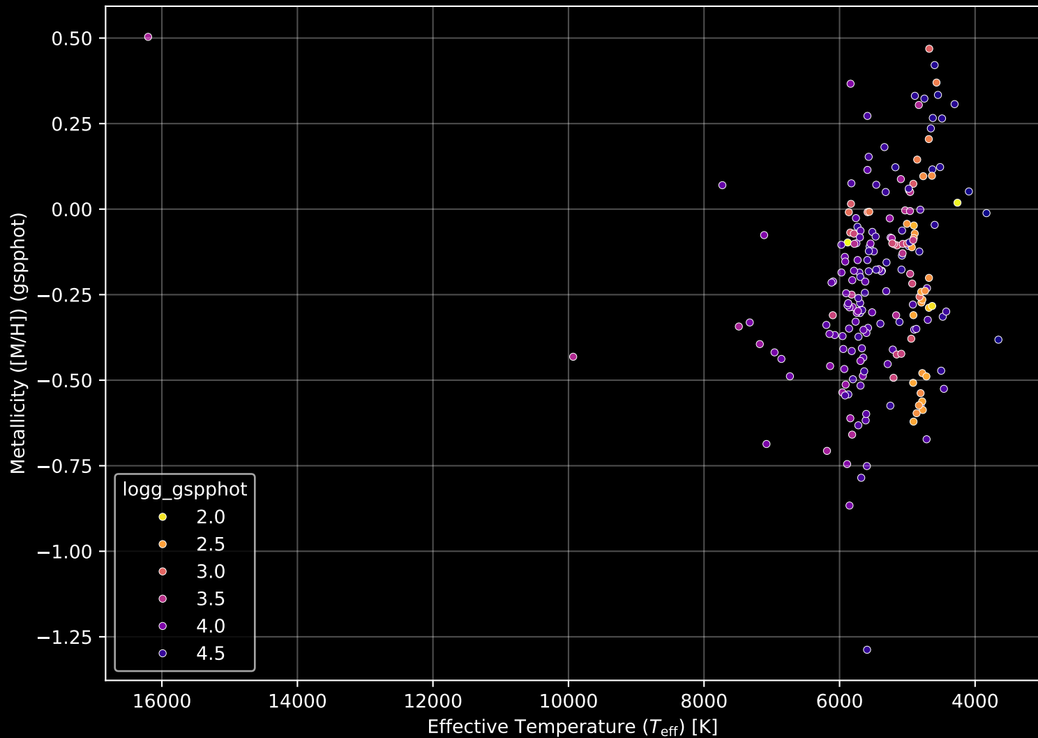
APOGEE DR17 Field: [193+34_MGA] Stellar Population Parameters (n= 203)
