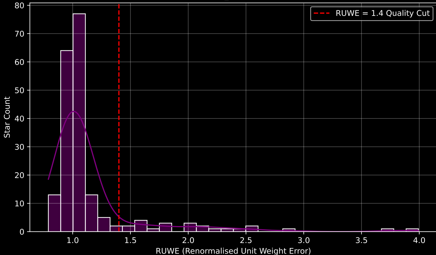
GAPOGEE DR17 Field [193+34_MGA] RUWE Distribution (n= 197)
