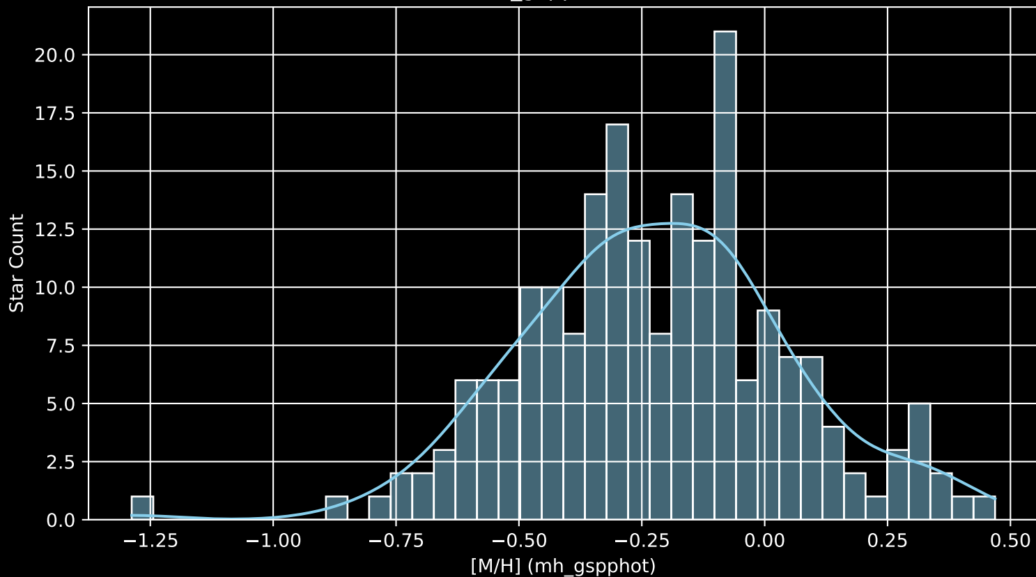
APOGEE DR17 Field: [193+34_MGA [M/H] (mh_gspphot) (n= 202)
