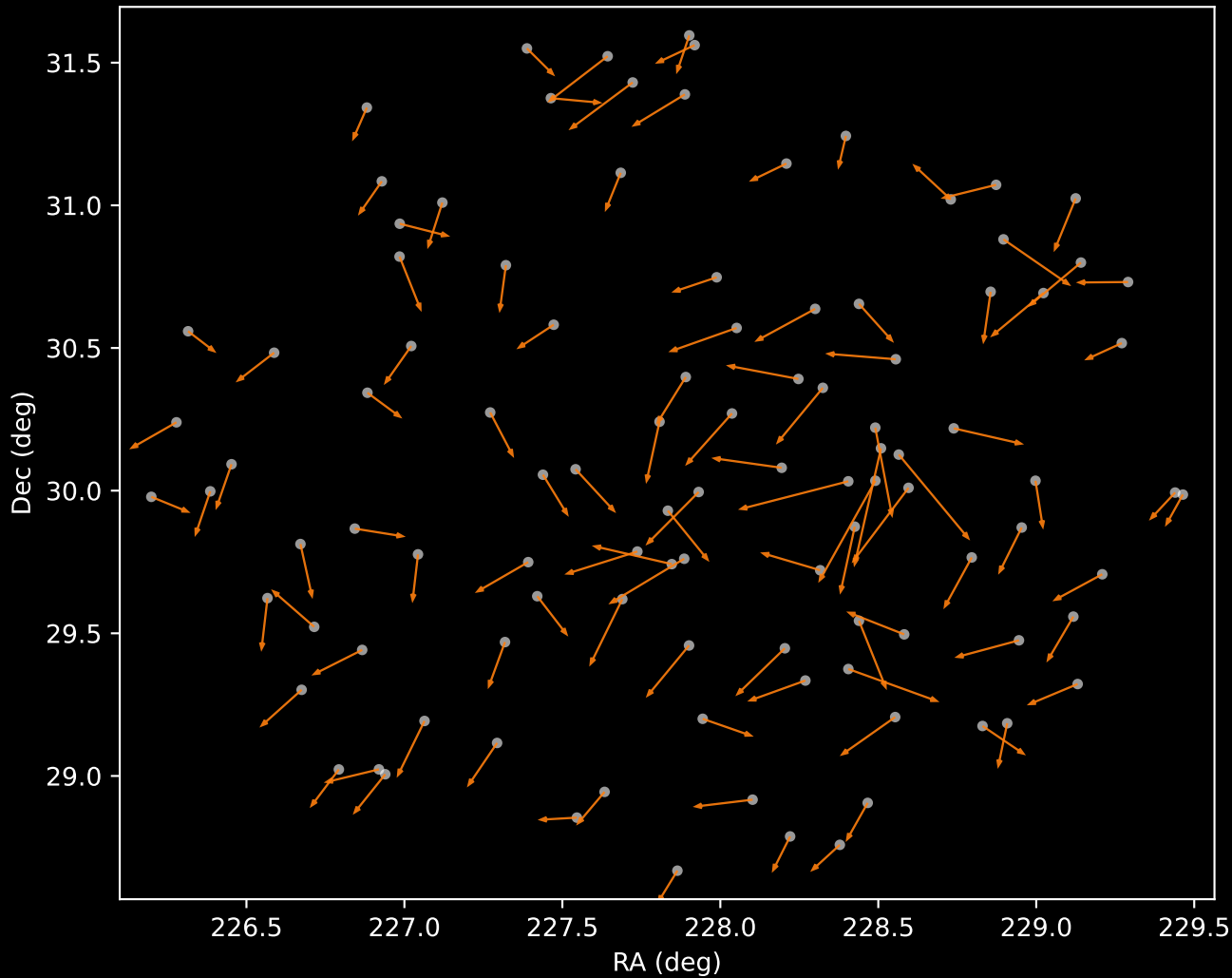
APOGEE DR17 Cluster 2 Proper Motion Vectors (n=104)
